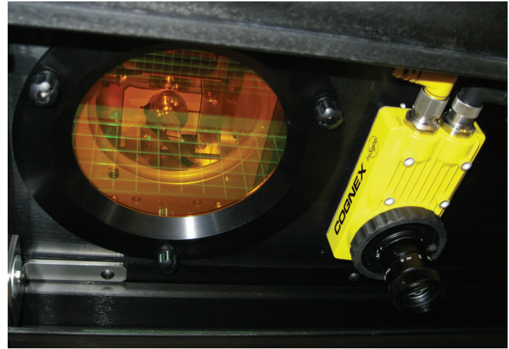
Our automated vision system enables the easy change of print registration positions.
